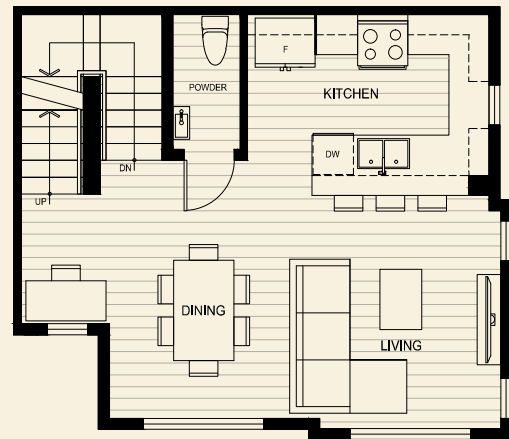
Second Level
